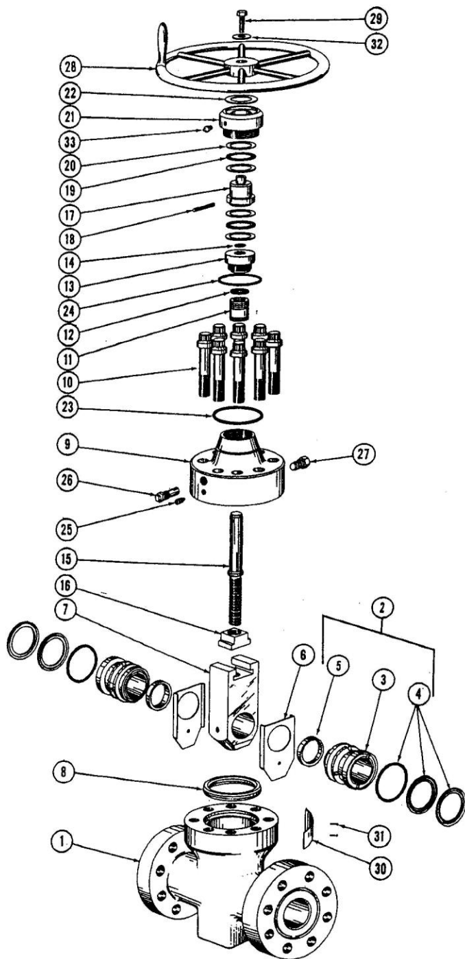
5,000 psi Type B Valve
