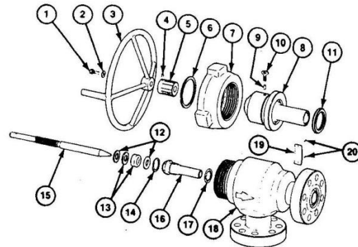
1" Maximum Orifice, 15,000 psi WP H2 Adjustable Choke
