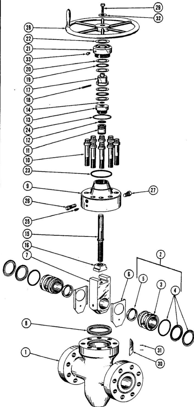
10,000 psi Type B Valve
