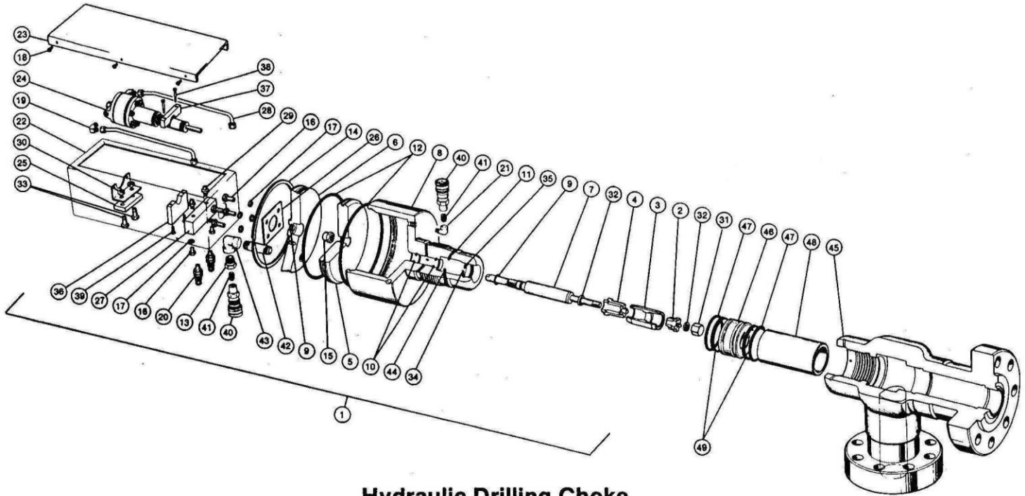
Hydraulic Drilling Choke
