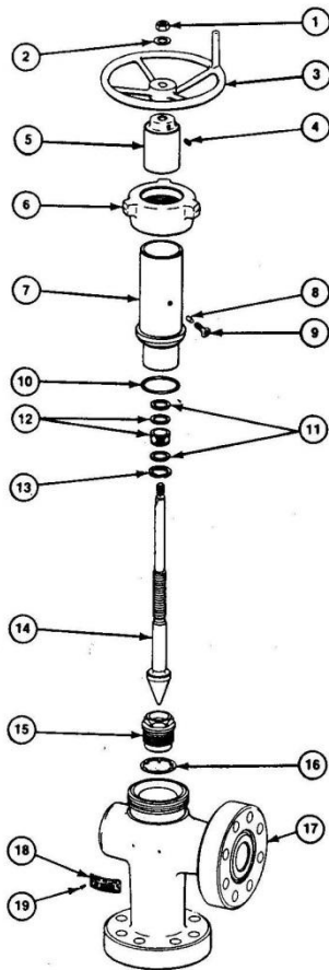
Typical 2000 through 10,000 psi WP H2 Adjustable Choke
